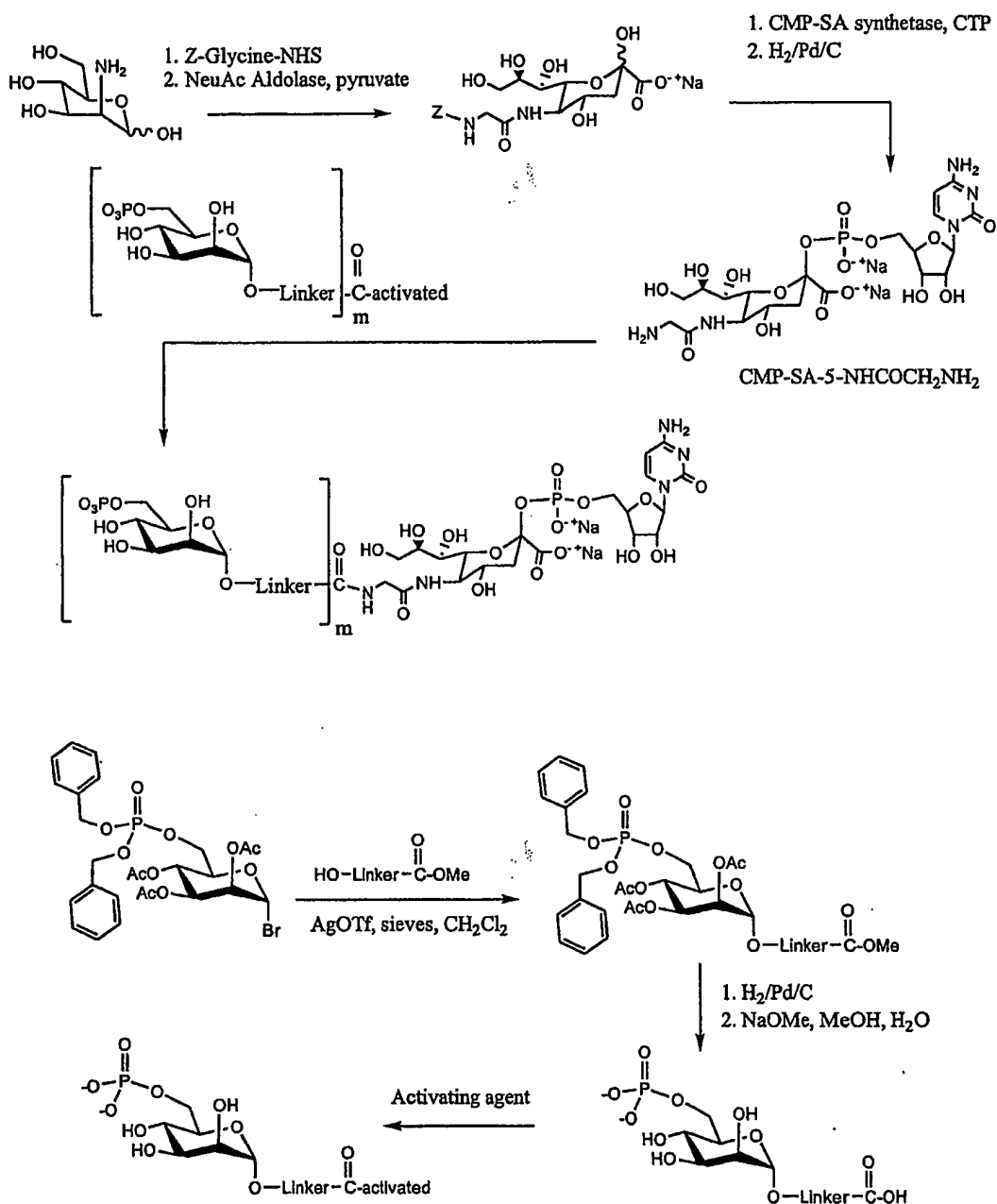
Scheme 15
